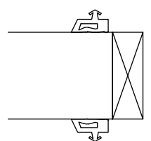
1 1/4" GLAZING
