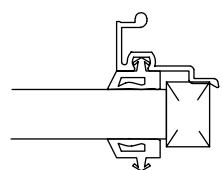
1/2" GLAZING
